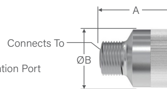
Plug Style
